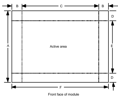
Figure 10 Active area of modules
