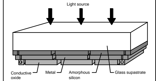
Figure 2 Module internal structure
