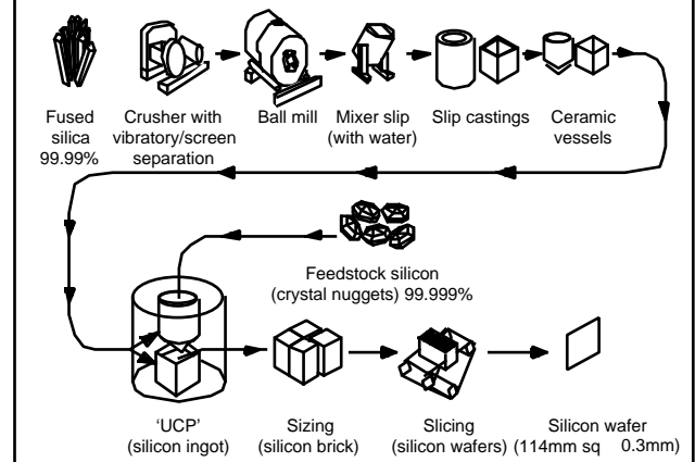
Figure 3 Cell production process
